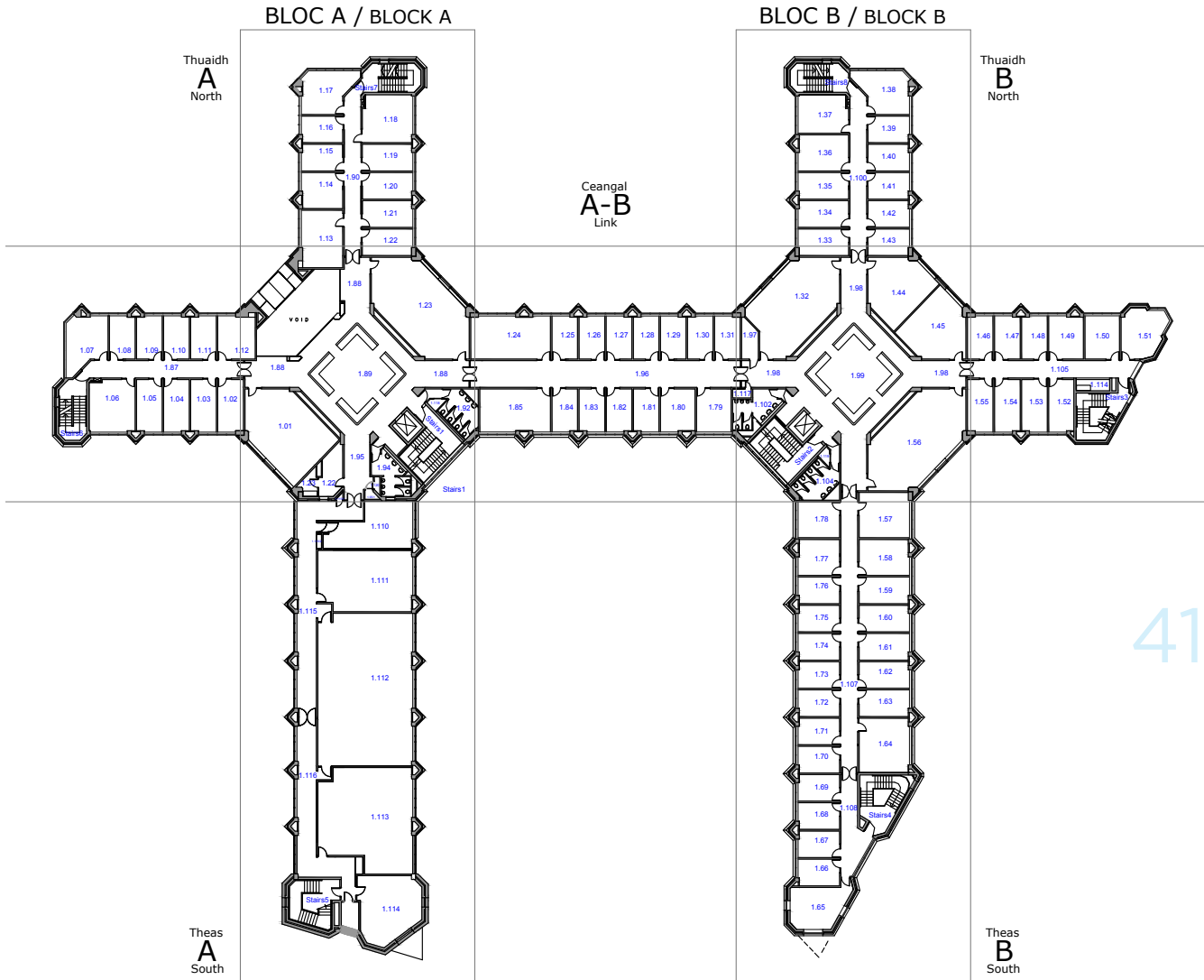
O'Rahilly Building First Floor Plan
