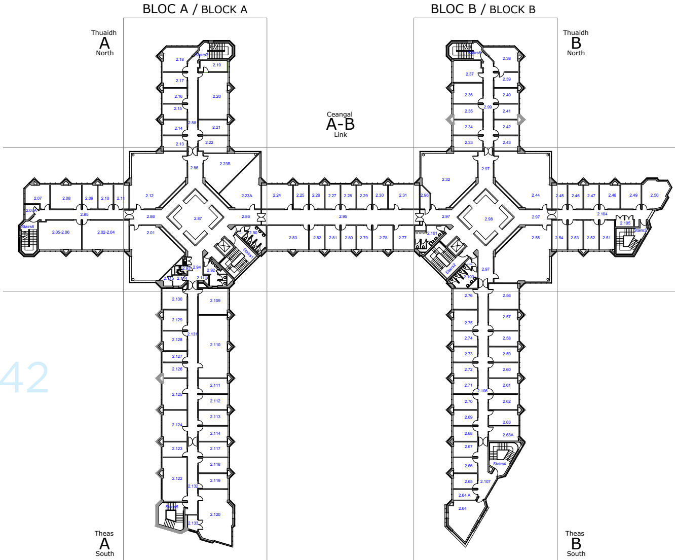
O'Rahilly Building Second Floor Plan
